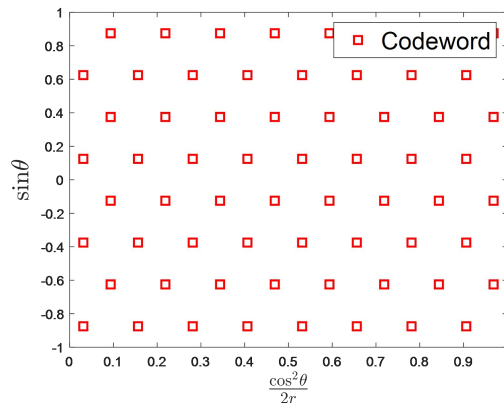
Fig. 5.15 Angle-displaced near-field codebook design method
