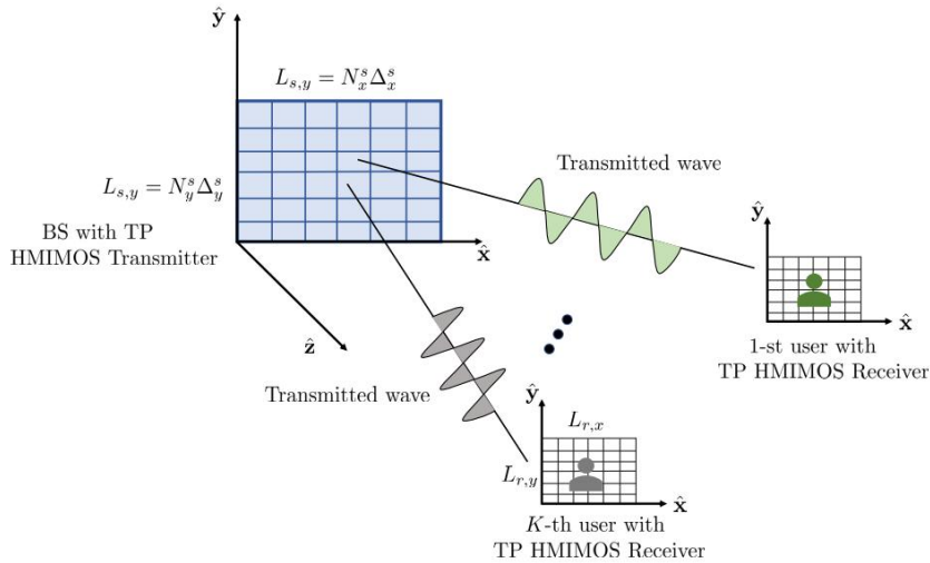
Fig. 4.20 Modeling of near-field multi-polarized spherical waves
