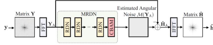
Fig. 5.4 MRDN-based channel estimation scheme
