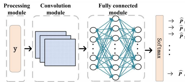
Fig. 5.18 Neural network structure for near-field beam training
