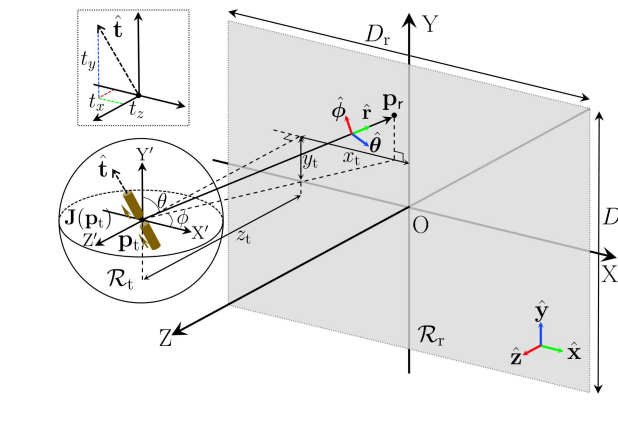
Fig. 6.2 Near-field positioning and attitude sensing.
