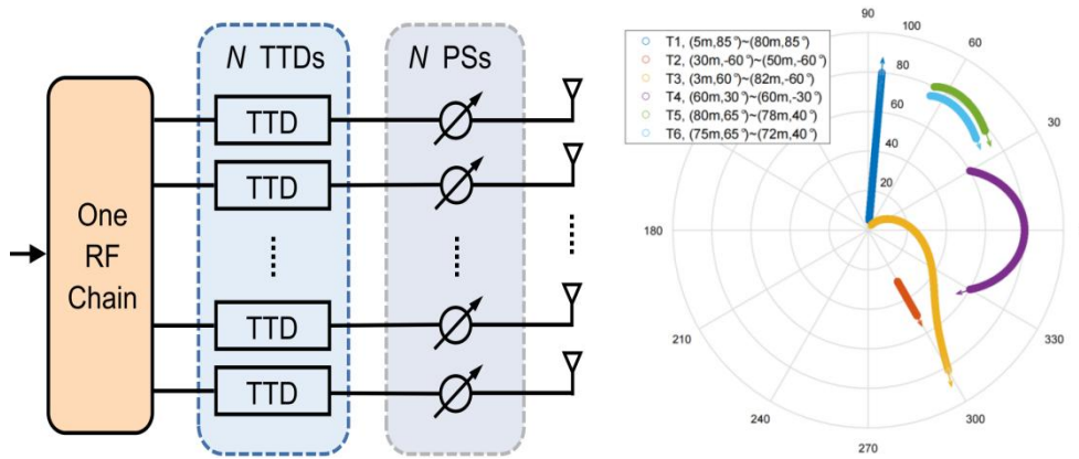
Fig. 6.12 Schematic diagram of near-field controllable beam squint.
