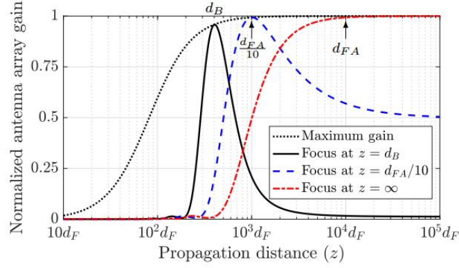
Fig. 3.7 Trend of beam gain with distance
