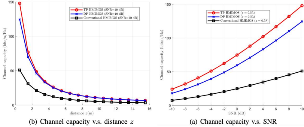
Fig. 3.5 Near-field tri-polarized channel capacity
