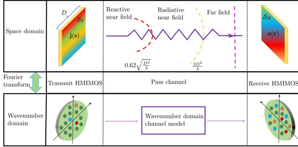
Fig. 3.20 Fourier plane wave expansion channel model
